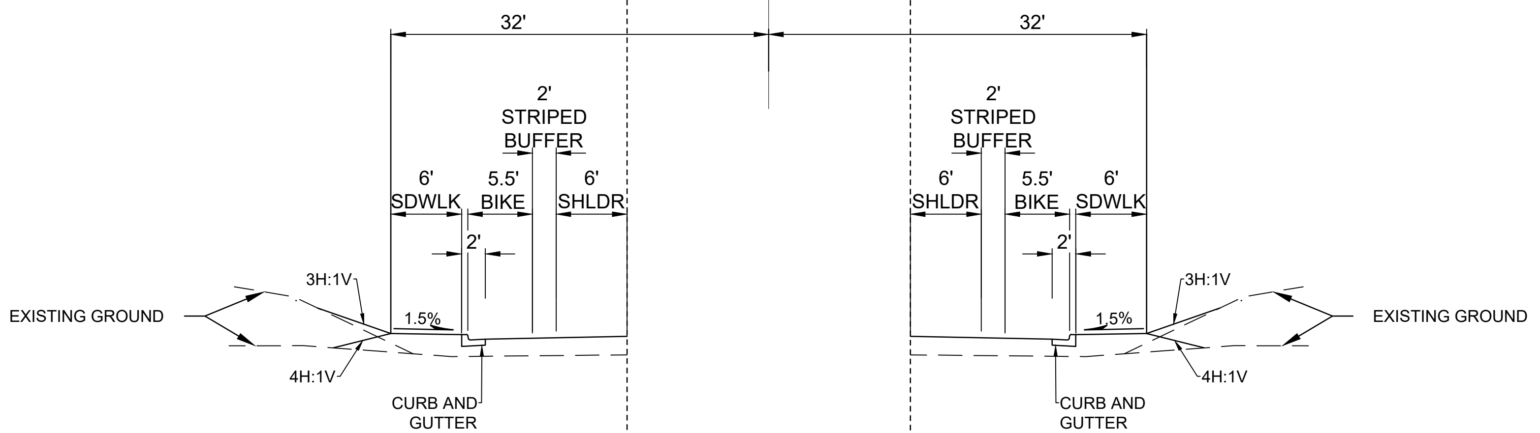
SEPARATED BIKE LANE OPTION
